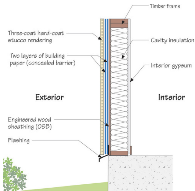
Figure 1: Two Layers of Building Paper —The two layers of building paper are significant in the performance of hardcoat stucco assemblies. The outer layer of building paper acts as bond break between the stucco and the inner layer of building paper permitting modest drainage of water between the two layers.
