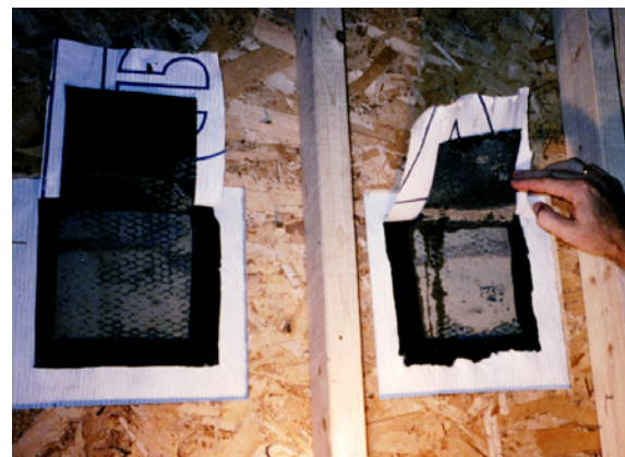
Photograph 7: Building Paper Bond Break —Traditional building paper is an excellent bond break between traditional hardcoat stucco and plastic building papers.
