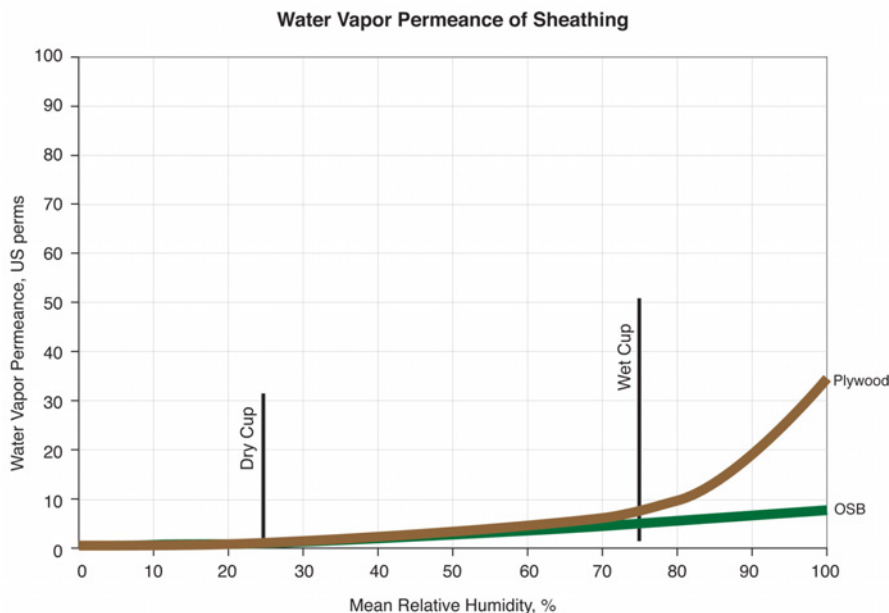
Figure 3: Permeance of Plywood vs OSB Sheathing —Note the “hockey stick” shape of the plywood curve. Hockey is good—remember that and life will be good. The upward rise allows the plywood to dry more readily than OSB when it gets wet.
