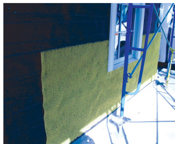
Photograph 8: Air Gap —The air gap does not have to be particularly big to be a big deal—3/8 inch (9 mm). One method of getting the air gap is to use a drainage mat between two layers of building paper. The gap allows redistribution of the moisture in both the stucco and the OSB sheathing.
