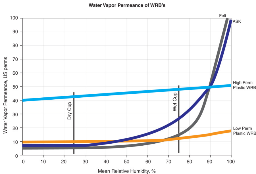
Figure 2: Permeance of Water Resistive Barriers (WRB's) —Debate rages within the building science community as to what the curves mean. The old guy in me intuitively believes that the shape of the curve describing the traditional building papers (WRB's) is “good.” And that the curve describing the “high perm” WRB is “not so good” and the curve describing the “low perm” WRB is “better but not as good as” the curve describing traditional building papers. I believe that if we could get a plastic building paper with a curve that mirrors the shape of the traditional building papers the product would “kick building science butt.”
