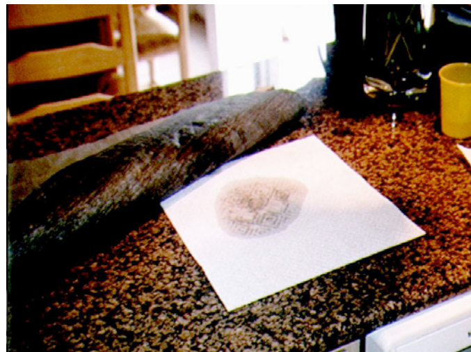
Photograph 7 (above left) - Joe Test 1 in 1995: It was not very predictive with new materials but pretty conclusive with field failures. That is my daughter helping me out. Photograph 8 (above right) – Failed Material: Weathering it seems was also important. Stuff seemed to be getting on to the stuff changing things . . .
