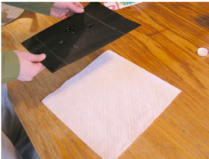
Photograph 5 (above left) – No Wet Spot: If the water beads up and does not wet the paper towel – it passes Joe Test 1. Photograph 6 (above right) – Nice House Gone Bad Stuff: In the case of the house we were looking at, the sample product removed from the wall failed Joe Test 1. Most products pass Joe Test 1 before they are installed. But all products that fail in the field seem to fail Joe Test 1.
