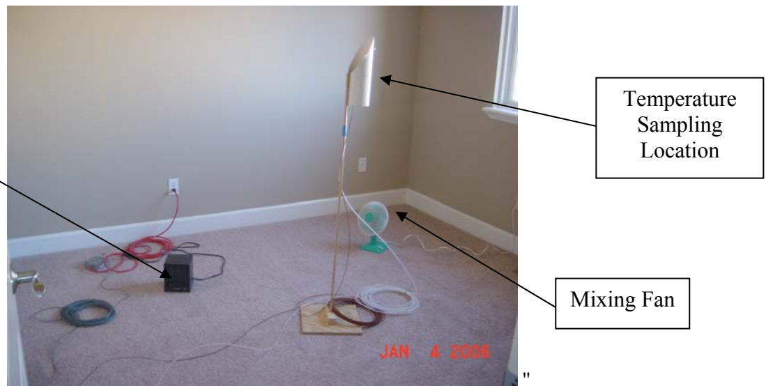
Figure 6. Tracer gas sampling point, temperature sensor, room air mixing and co-heating set-up.
