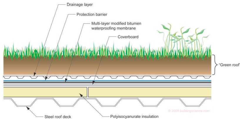
Figure 2: Bad Green Roof —The insulation is under the membrane. This is bad. The insulation can collapse and loose support for the membrane. The membrane can tear and leak. The reason for this bad design choice is often a preoccupation with the "greenness" of the blowing agent of the rigid insulation. Successful green roofs have historically used extruded polystyrene (XPS). XPS can get wet and still perform. The blowing agent of XPS is arguably not the "greenest of the green." Unproven "green" blowing agents used with polyiso-cyanurate insulation seem attractive at first blush, but insulation assemblies need to be protected from water and hence the location under the membrane and the structural loading of the overbuild assembly needs to be taken into account.
