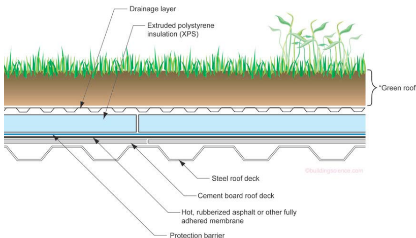
Figure 3: Good Green Roof —The insulation is over the top of the membrane. This is good. This configuration has a multi-decade track record.
